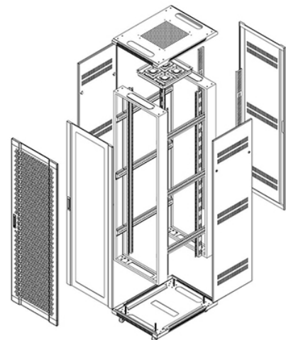
Structure drawing
