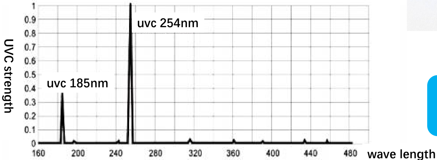
Relative spectral power distribution of ozone germicidal uv lamp
