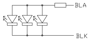
Backlight Circuit (No. of LEDs = 3pcs) Scale=free
